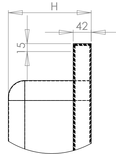
DETAIL M SCALE 1 : 6
